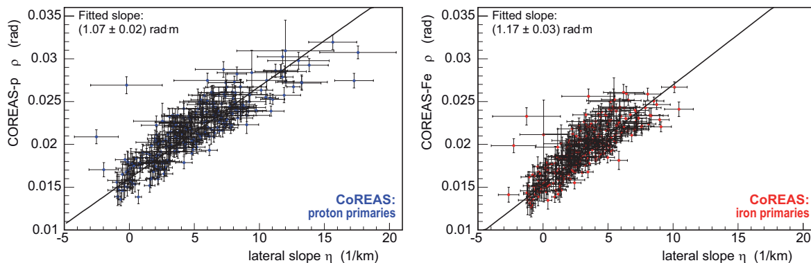
Figure 12. Correlation of the cone angle \rho and the slope parameter \eta of the lateral distribution for the CoREAS proton simulations (left) and the iron simulations (right). As expected, showers with a steeper lateral distribution (large \eta ) also have a steeper radio wavefront (large \rho ), since both are affected by the distance to the shower maximum.
