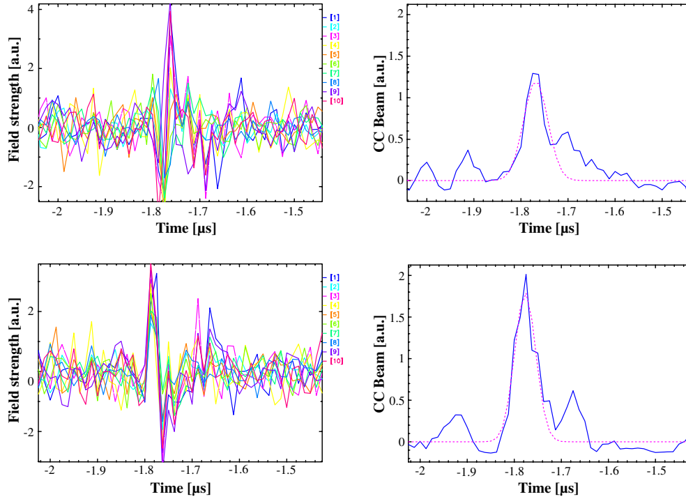
Fig. 3. Event example: Upper panels: Signals of the individual antennas and result of the beam-forming (full line: CC-beam; dotted line: Gaussian fit) based on shower observables reconstructed by Grande; Lower panels: Signals of the individual antennas and result of the optimized beam-forming in order to maximize the radio coherence.
