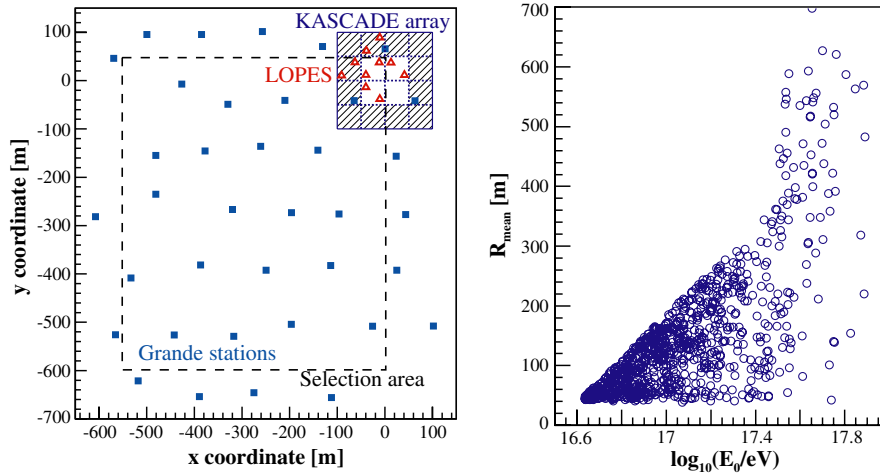
Fig. 1. Left panel: Sketch of the KASCADE-Grande experiment. The main detector components are the KASCADE array and the Grande stations. The location of the 10 LOPES radio antennas is also displayed. Right panel: Distribution of the selected candidate events (862 events) with respect to primary energy (obtained by Grande reconstruction) and mean distance of the shower axis to the radio antennas. The selection is based on cuts of Eq. (2), see text.
