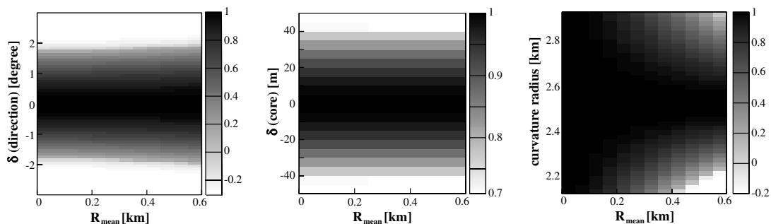
Fig. 2. Analytically estimated sensitivity of the (cross-correlation) CC-beam to the variation of the shower direction \delta(\text{direction}) , the shower core position \delta(\text{core}) , and the radius of curvature of the radio front in dependence of R_{\text{mean}} for the LOPES-10 configuration, assuming a monochromatic point source emitting at 60 MHz.
